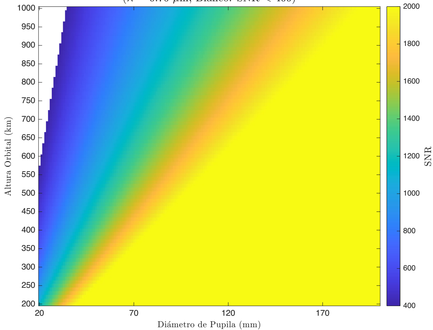
SNR - Cassegrain - Detector 1 ( \lambda = 0.76 \mu\text{m} , Blanco: \text{SNR} < 400 )
